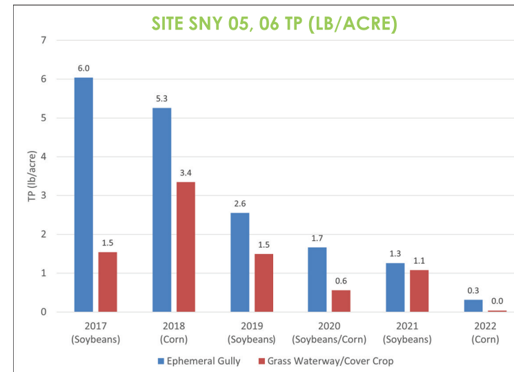
▲ Figure 8 (Site SNY 05, 06) Despite the installation of terraces at the control plot in 2020, the phosphorus loads leaving the grass waterway and cover crop combination were still lower.
