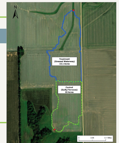
► Figure 5 (Site SNY 05, 06) Treatment and control drainage areas.
